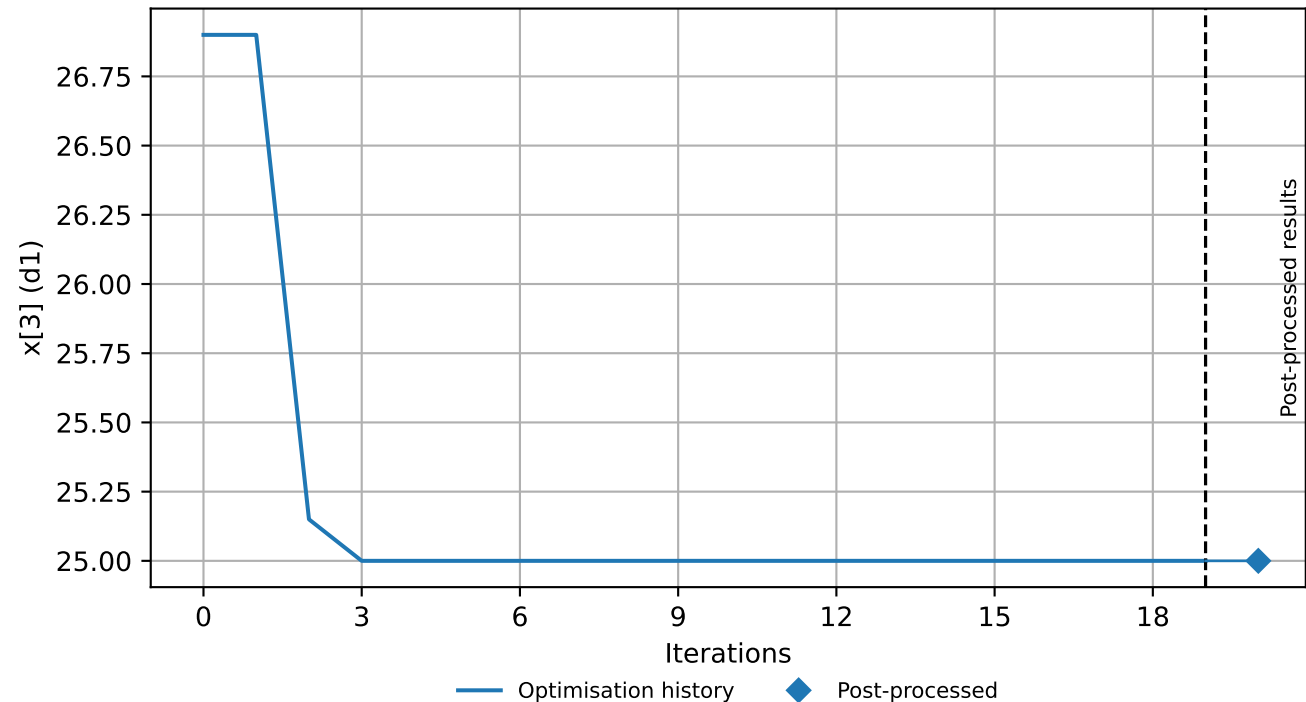
SLP Design variable convergence: d1
